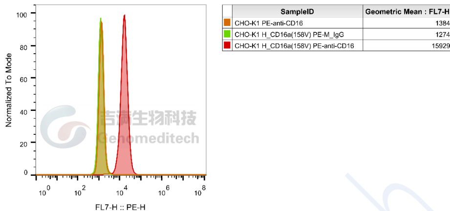
Figure 1 | H_FCGR3A(CD16a) 158V CHO-K1 Cell Line was determined by flow cytometry using PE anti-human CD16 Antibody (BioLegend/302007).
